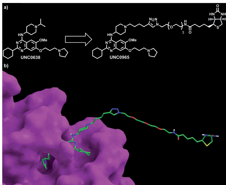
Figure 1. Design of UNC0965. a) G9a-UNC0638-SAH co-crystal structure (PDB ID: 3RJW) was previously solved and demonstrated that the N -isopropyl group of UNC0638 is solvent exposed. We took advantage of this chemical handle and designed the biotinylated derivative UNC0965. b) Docking of UNC0965 into the G9a crystal structure predicts a similar binding mode as UNC0638. Importantly, the biotin moiety of UNC0965 is solvent exposed and suitable for streptavidin capture.
